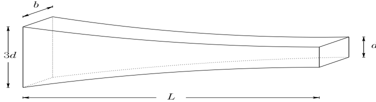
FIGURE 5. Smoothly varying cross-section beam.
