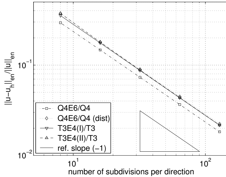
Fig. 4. Fully constrained block. Polynomial load test. Energy-norm convergence rate for \underline{u} .
