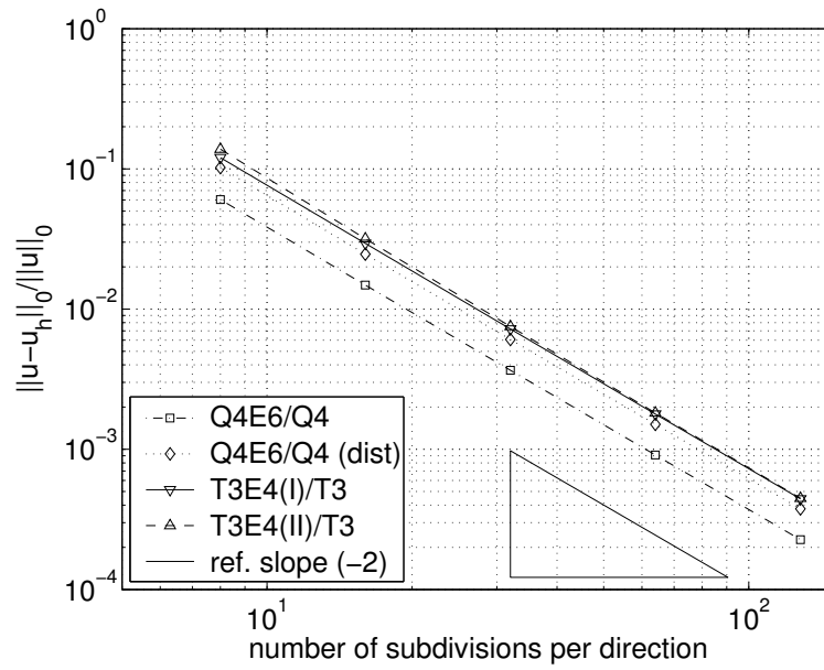
Fig. 5. Fully constrained block. Trigonometric load test. L^2 -norm convergence rate for u .
