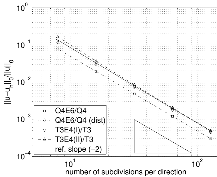
Fig. 2. Fully constrained block. Polynomial load test. L^2 -norm convergence rate for \underline{u} .
