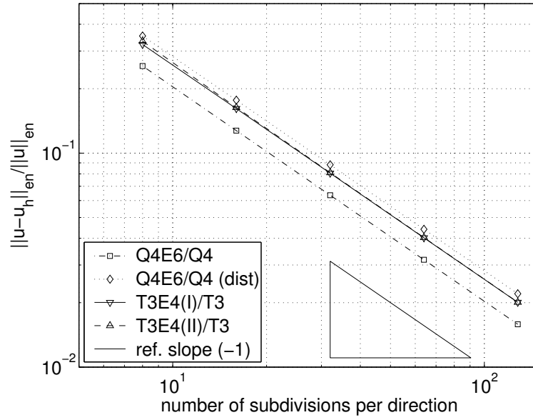
Fig. 7. Fully constrained block. Trigonometric load test. Energy-norm convergence rate for \underline{u} .
