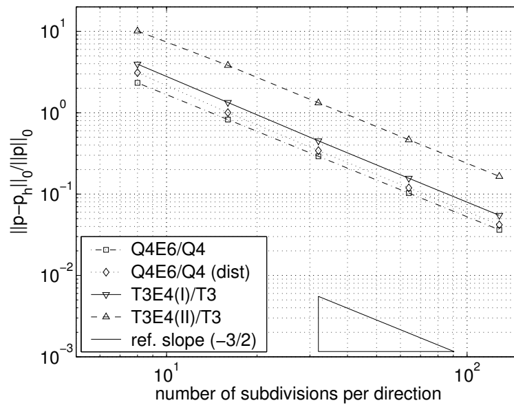
Fig. 6. Fully constrained block. Trigonometric load test. L^2 -norm convergence rate for p .
