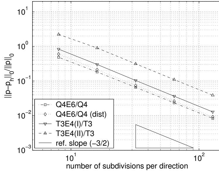
Fig. 3. Fully constrained block. Polynomial load test. L^2 -norm convergence rate for p .
