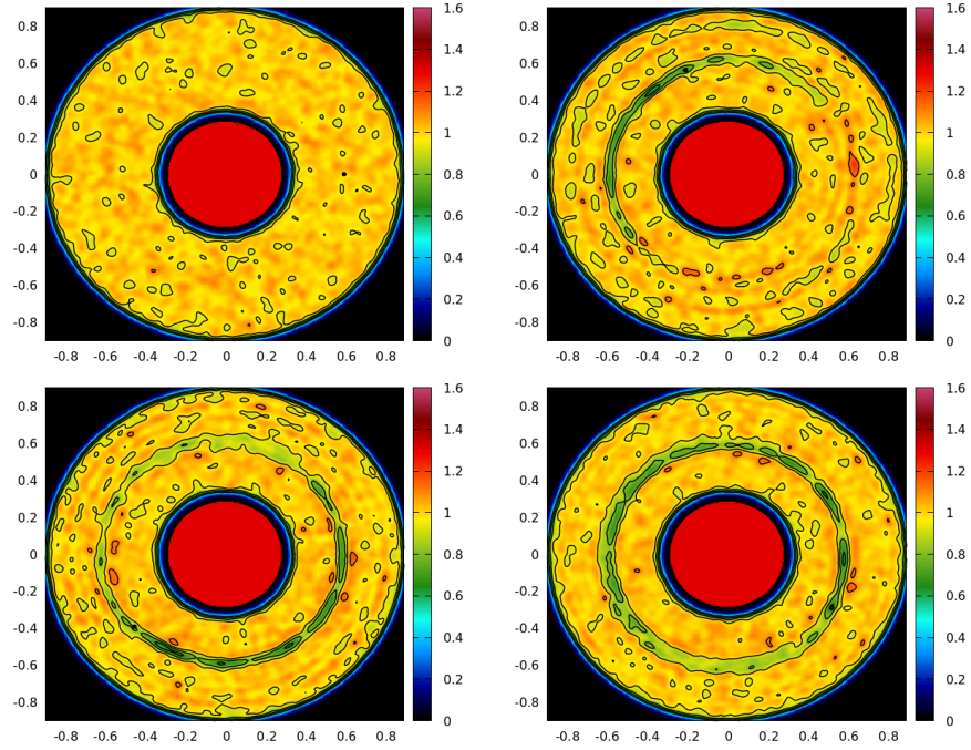
FIGURE 2. Time history of the spatial numerical density \rho_{N^0,\varepsilon}^n at instants t = 0 s, t = 6.0 \times 10^5 s, t = 1.2 \times 10^6 s, t = 1.8 \times 10^6 s, starting from the image at the top left, proceeding from left to right and from top to bottom. The axis are scaled according to the length L^0 = 2 \times 10^8 m.
